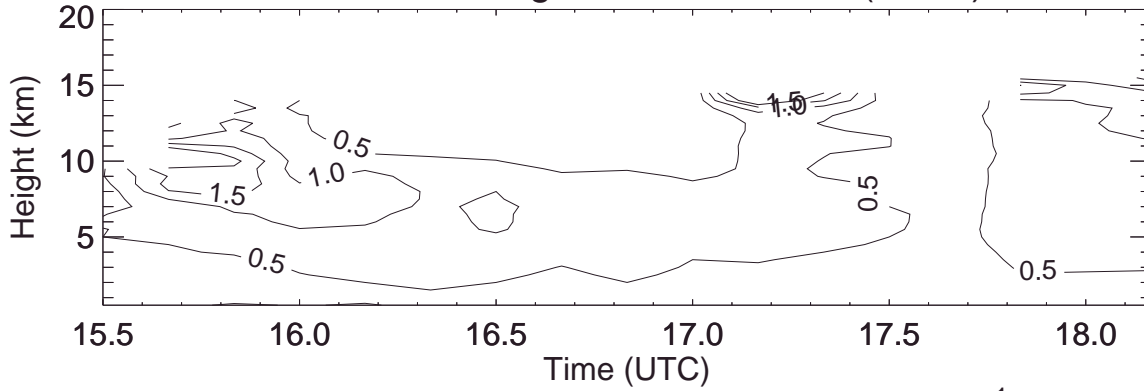
990207: Maximum Vertical Air Motion ( \text{m s}^{-1} )
