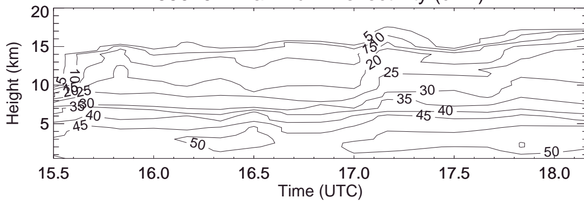
990207: Maximum Reflectivity (dBZ)
